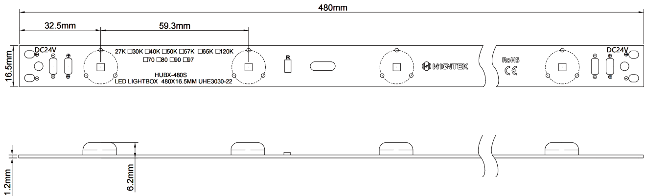
Figure 2. Mechanical Dimensions for HIGNTEK HUB-480SA-024008.
