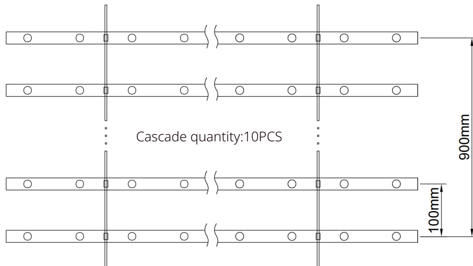
Figure 3. Assembly drawing for HIGNTEK HUB-480SA-024008.
