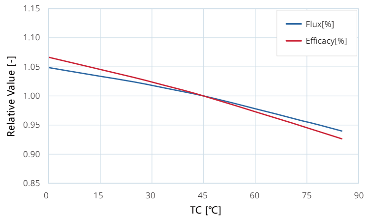
Figure 1. Typical normalized light output vs. T_c temperature for HIGNTEK HUB-480SA-024008 at DC24V.
