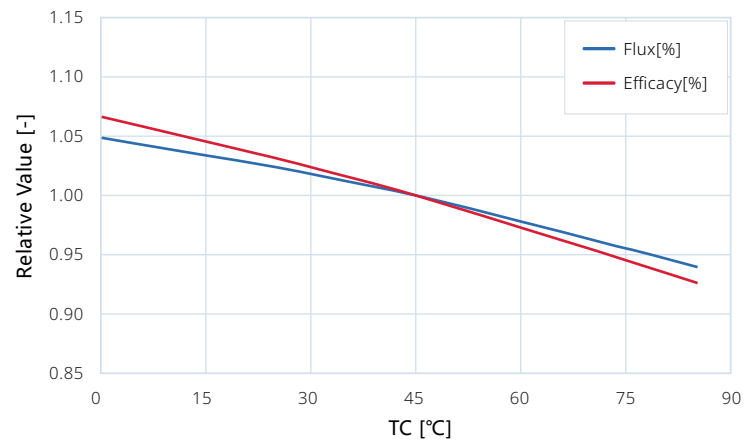
Figure 1. Typical normalized Flux and Efficacy vs. T_c temperature for HIGNTEK HUB-1130SA-012016 at DC12V.
