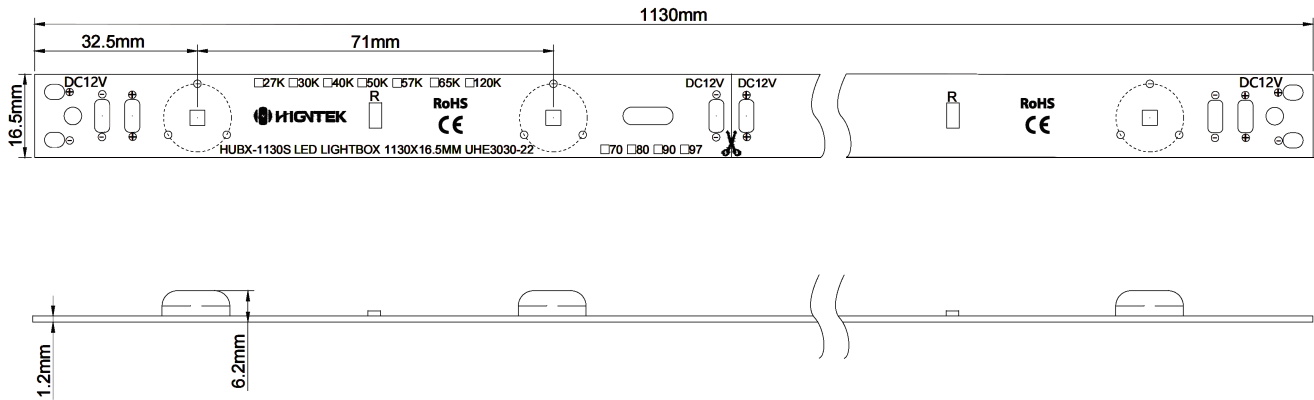
Figure 2. Mechanical Dimensions for HIGNTEK HUB-1130SA-012016.
