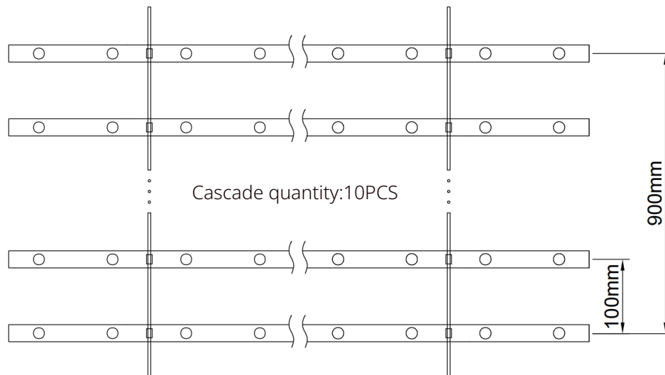
Figure 3. Assembly drawing for HIGNTEK HUB-1130SA-012016.
