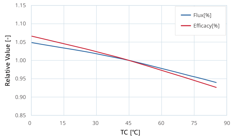
Figure 1. Typical normalized Flux and Efficacy vs. T_c temperature for HIGNTEK HUS-008SA-012128 at DC12V.
