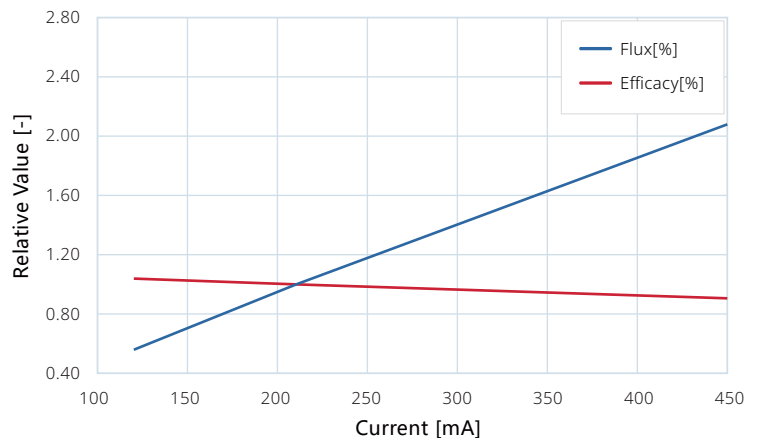
Figure 2. Typical normalized Flux and Efficacy vs. Current for HIGNTEK HUL-280SA-024024.
