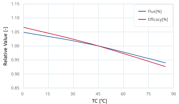
Figure 1. Typical normalized Flux and Efficacy vs. T_c temperature for HIGNTEK HUL-280SA-024024.
