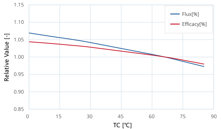
Figure 1. Typical normalized Flux and Efficacy vs. T_c temperature for HIGNTEK HUO-121SA-024008.
