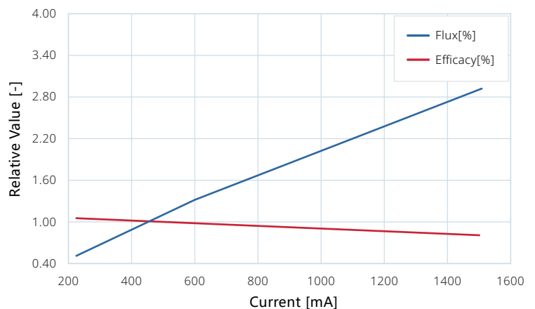
Figure 2. Typical normalized Flux and Efficacy vs. Current for HIGNTEK HUO-121SA-024008.
