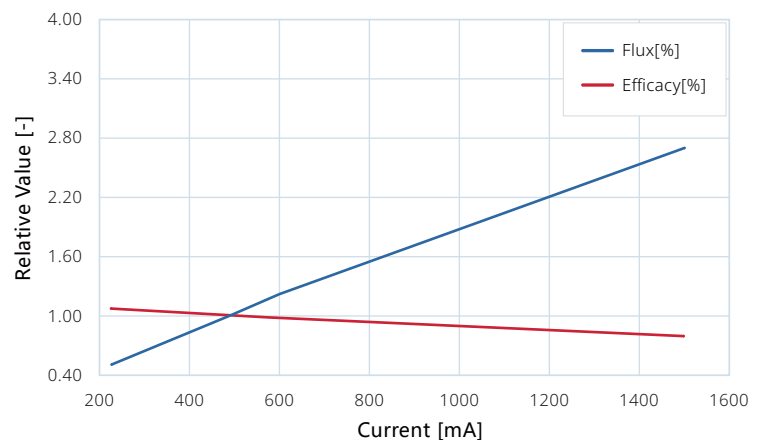
Figure 2. Typical normalized Flux and Efficacy vs. Current for HIGNTEK HUO-146SA-036012.
