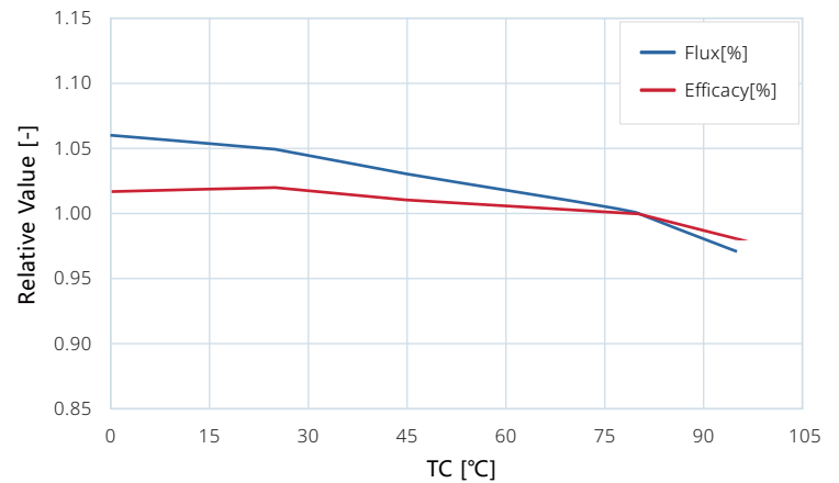
Figure 1. Typical normalized Flux and Efficacy vs. T_c temperature for HIGNTEK HUO-146SA-036012.
