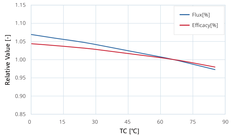
Figure 1. Typical normalized Flux and Efficacy vs. T_c temperature for HIGNTEK HUO-172SA-036012.
