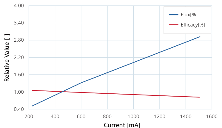
Figure 2. Typical normalized Flux and Efficacy vs. Current for HIGNTEK HUO-172SA-036012.
