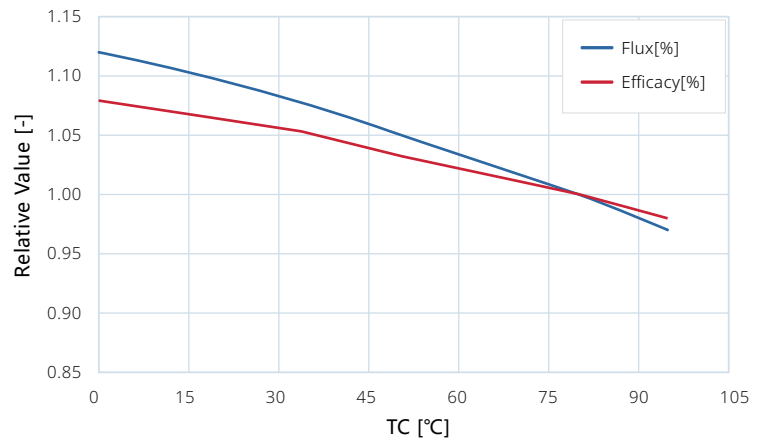
Figure 1. Typical normalized Flux and Efficacy vs. T_c temperature for HIGNTEK HUO-172SA-036024.
