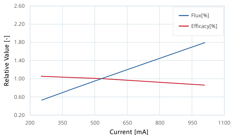
Figure 2. Typical normalized Flux and Efficacy vs. Current for HIGNTEK HUO-172SA-036024.
